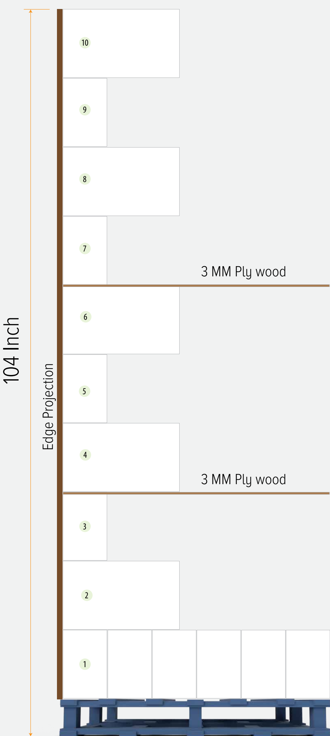
40" Feet Container
